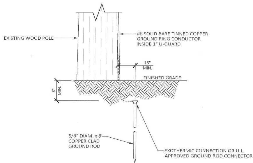
1 SINGLE POINT RADIAL GROUND DETAIL
