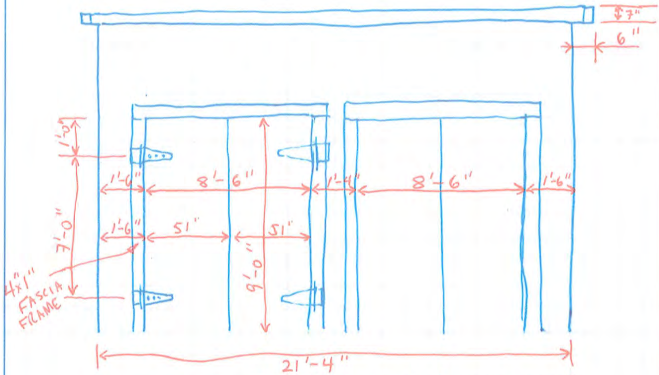
FRONT VIEW (LOOKING EAST)
