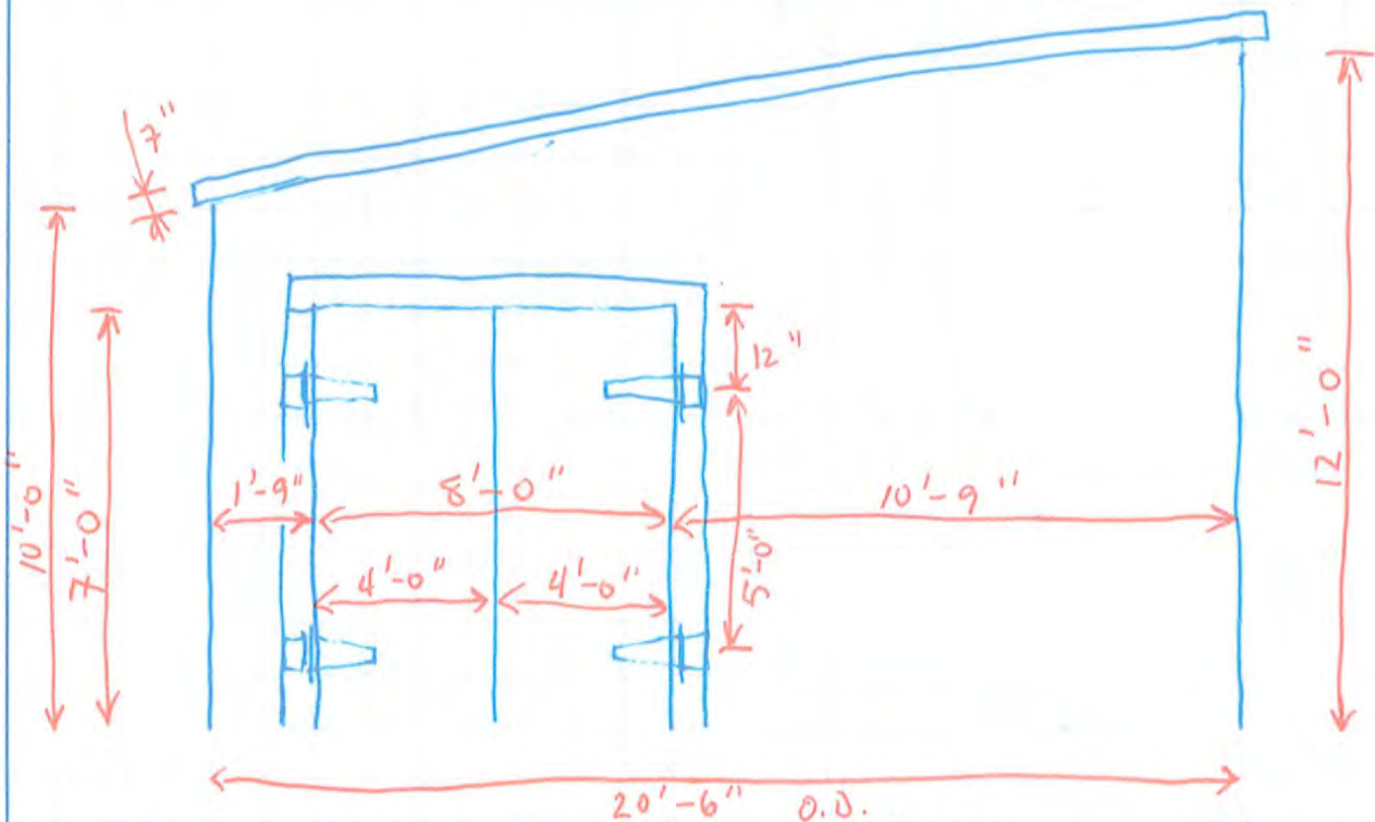
SIDE VIEW (LOOKING SOUTH)
