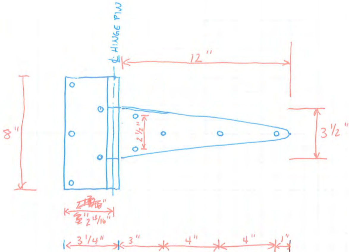
TYPICAL HINGE DETAIL — (12) TOTAL HINGES —
