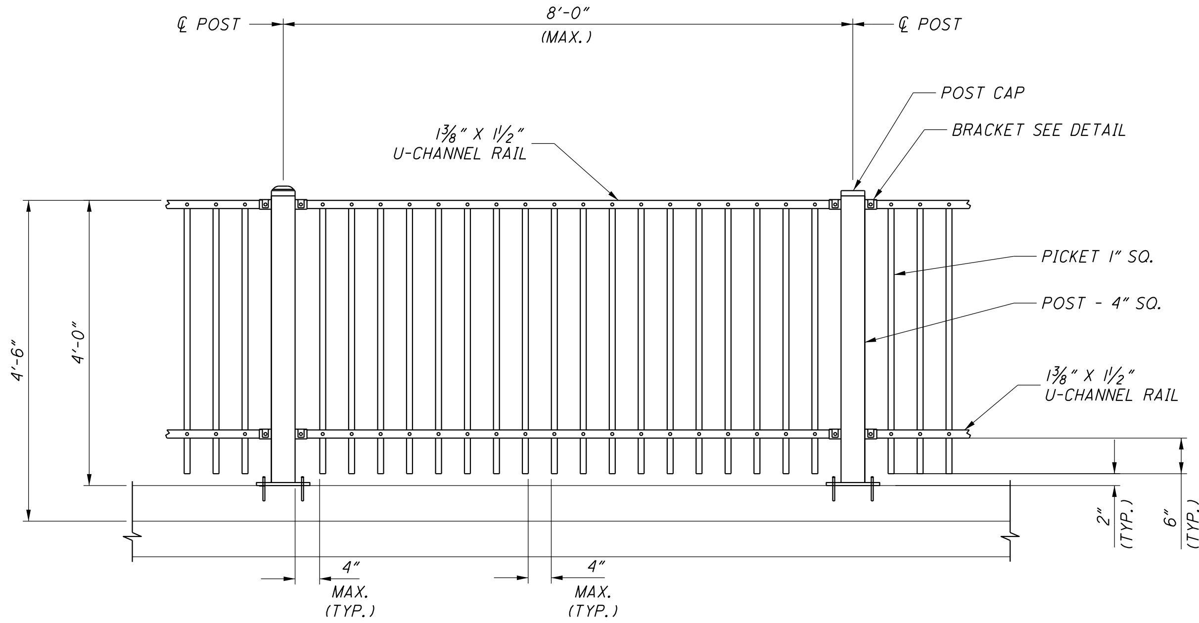
FENCE ELEVATION
