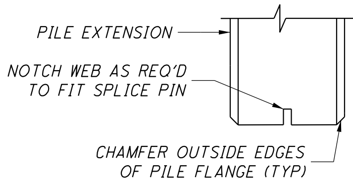
NOTCH DETAIL
