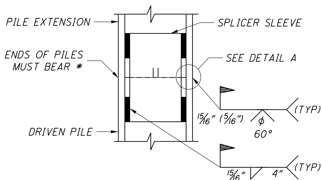
ALTERNATIVE SPLICE DETAILS
