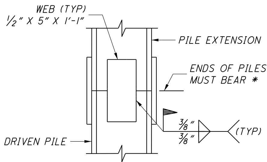
SPLICE DETAILS
