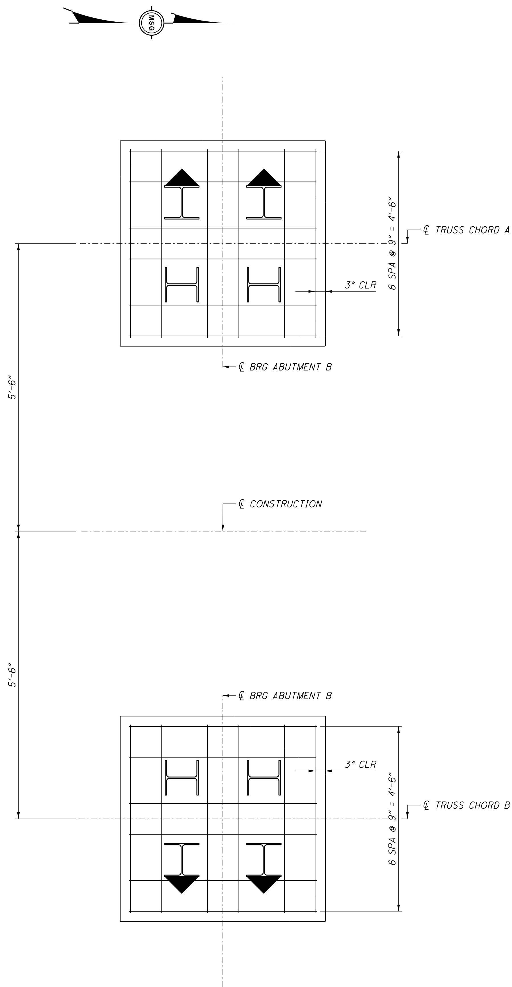
BOTTOM MAT REINFORCING
