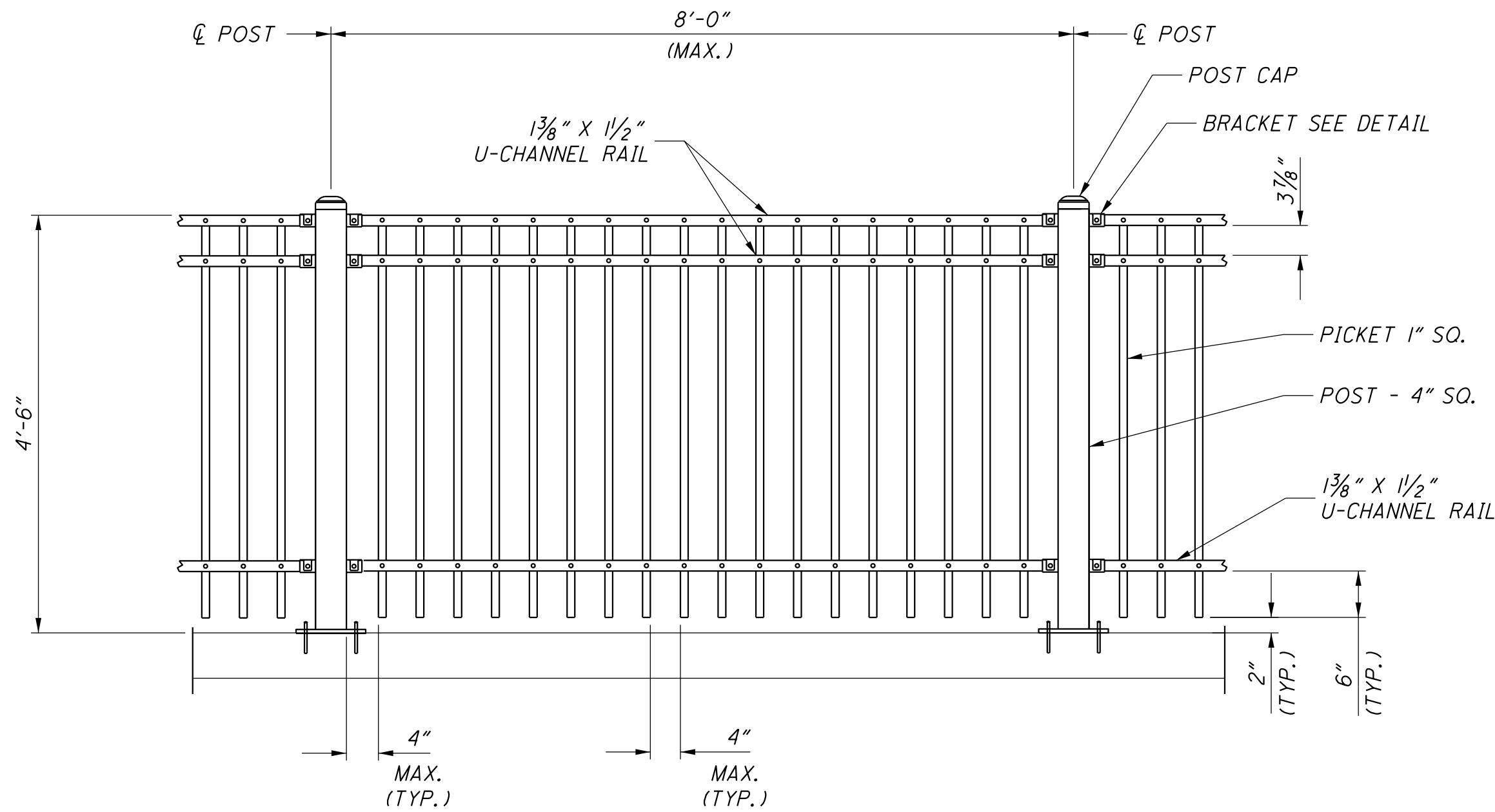
FENCE ELEVATION
