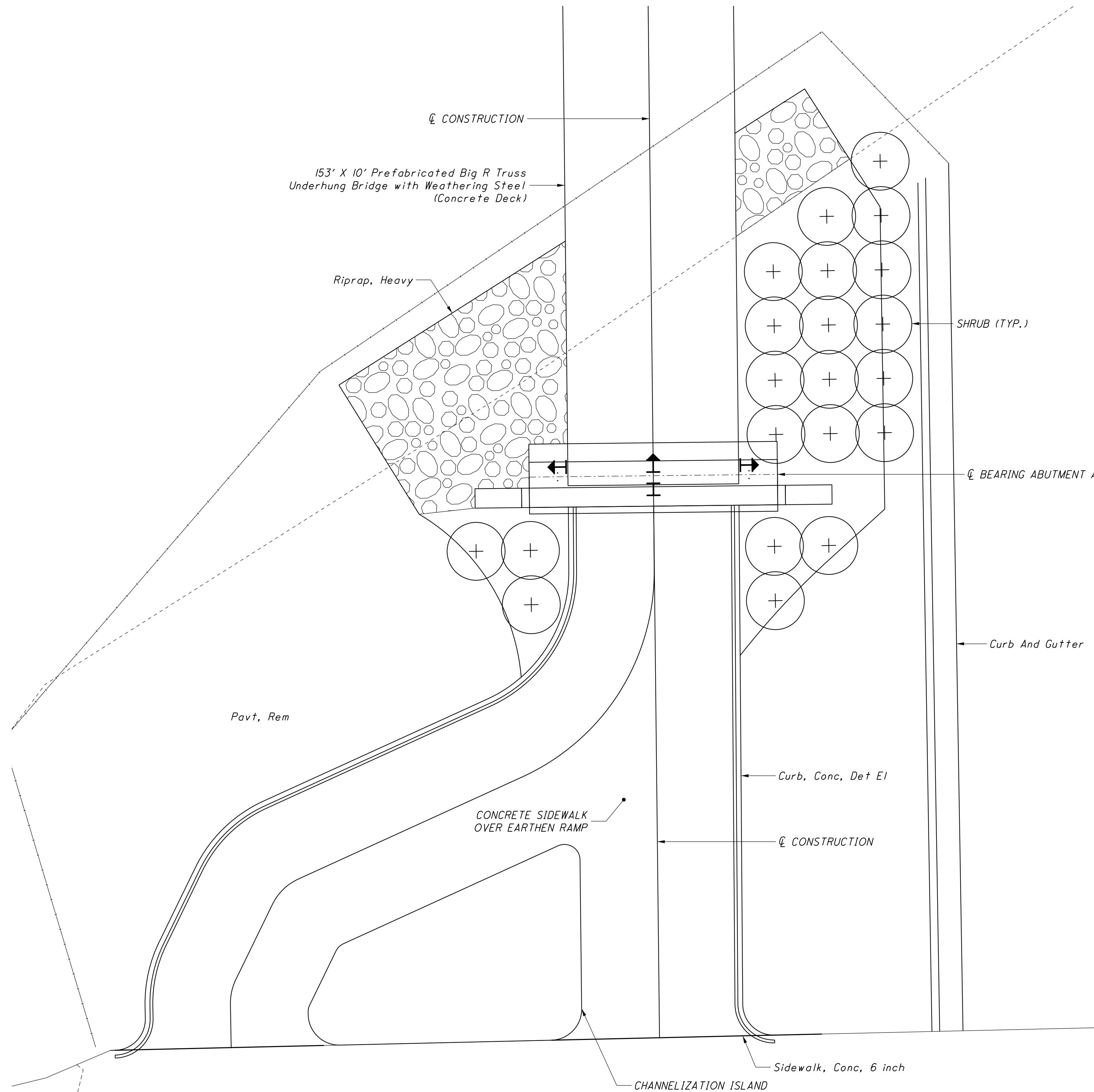
APPROACH PLAN SCALE: 1" = 20'-0"
