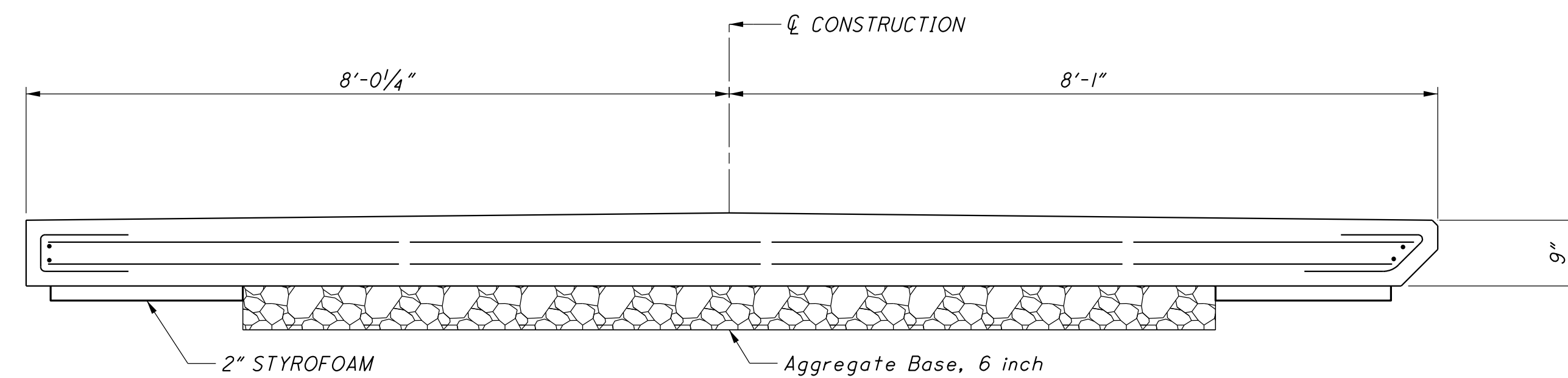
OVERLOOK #2 SECTION G-G
