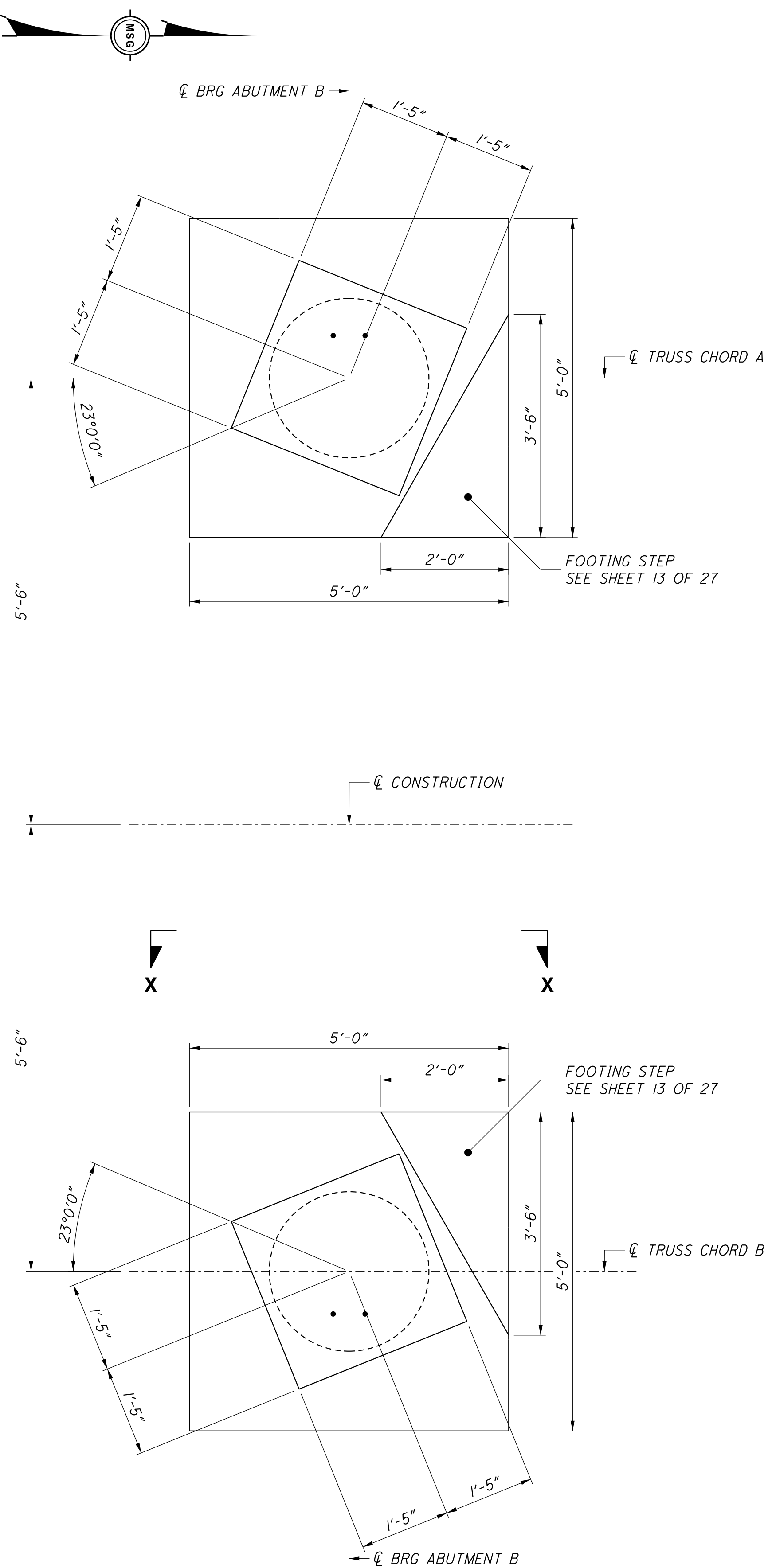
ABUTMENT B FOOTING PLAN
