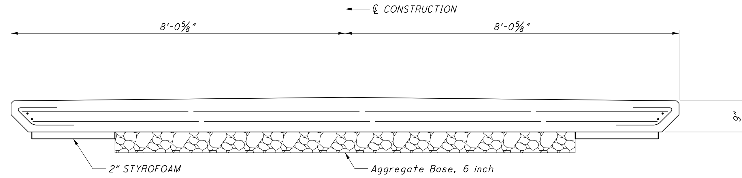
OVERLOOK #2 SECTION F-F
