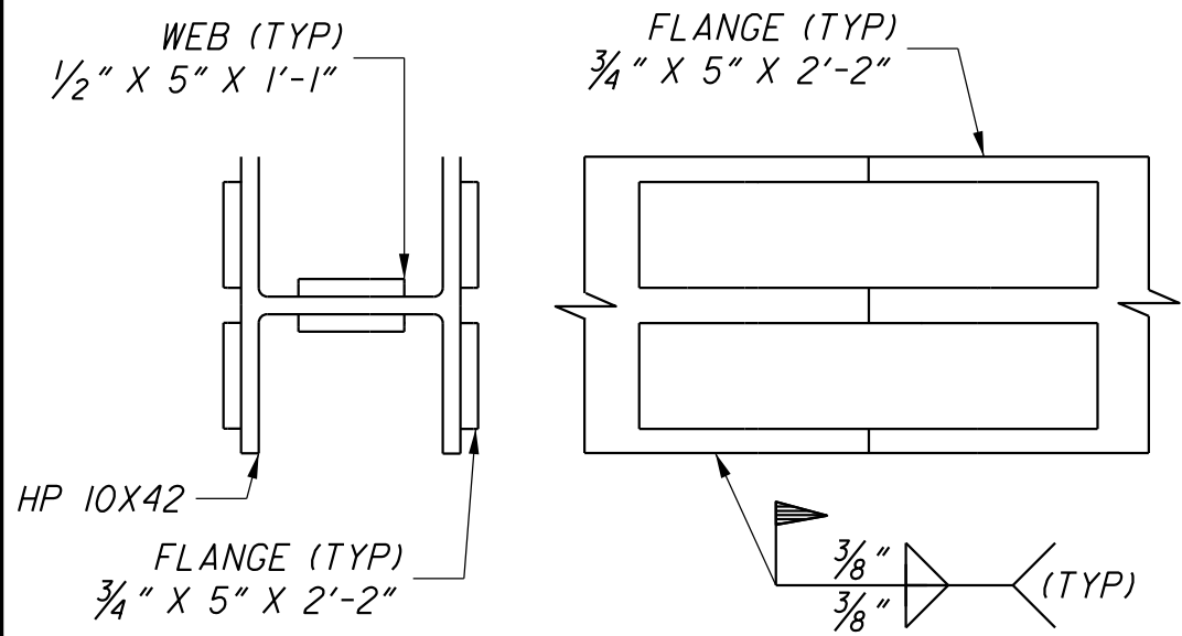
SPLICE DETAILS
