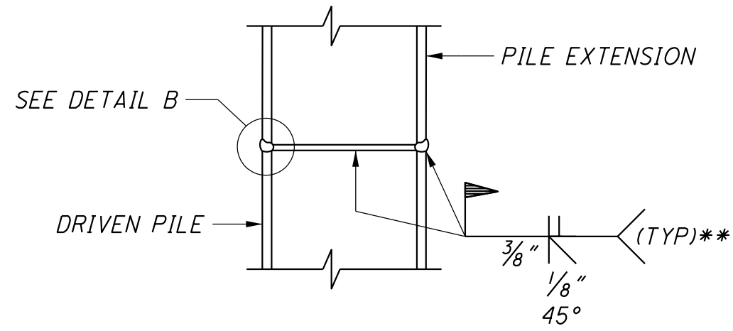
SPLICE DETAILS
