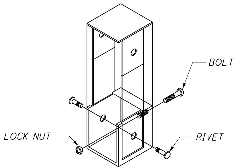
FENCE ELEVATION
