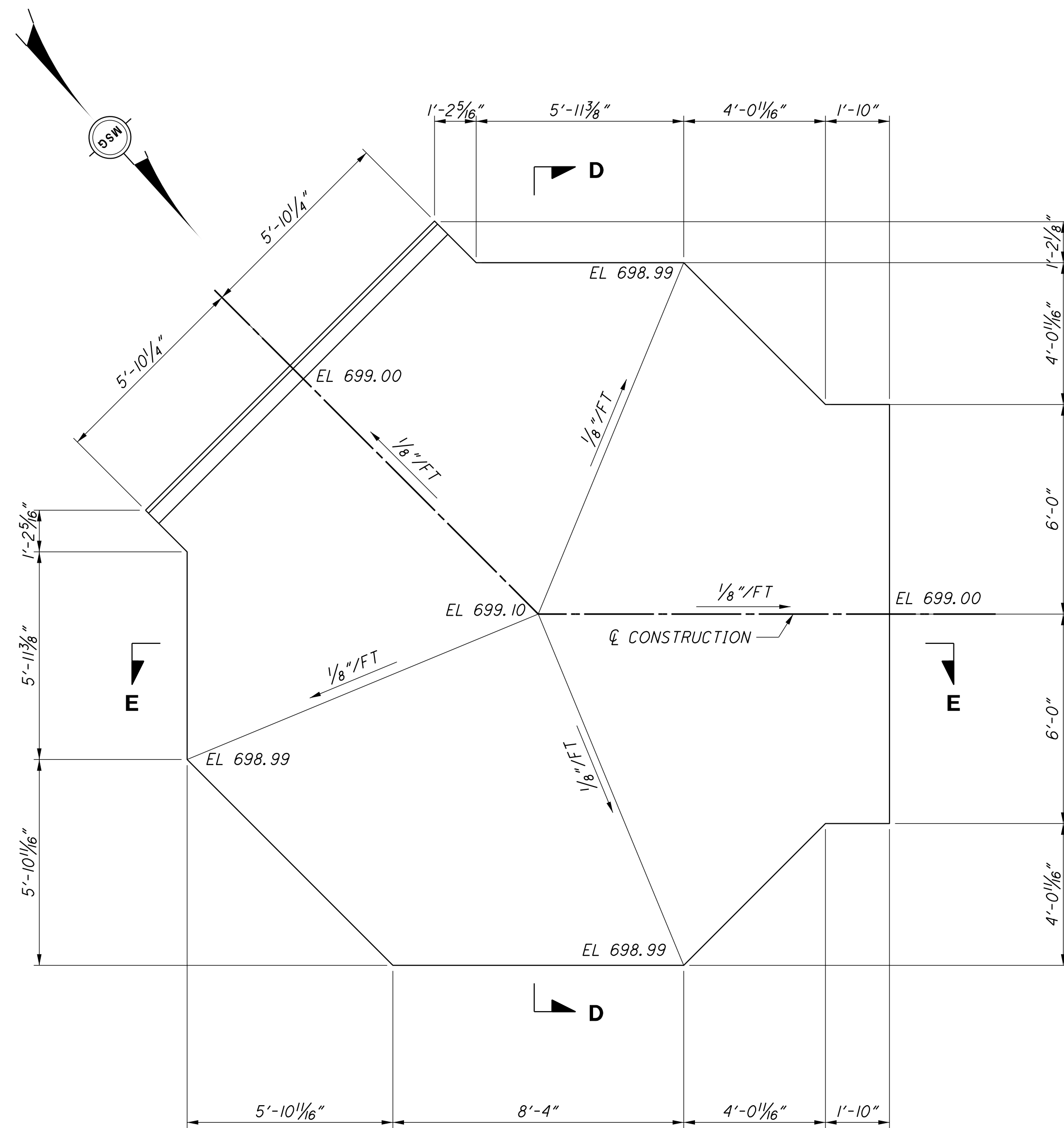
SLAB PLAN SCALE: \frac{3}{8}" = 1'-0"
