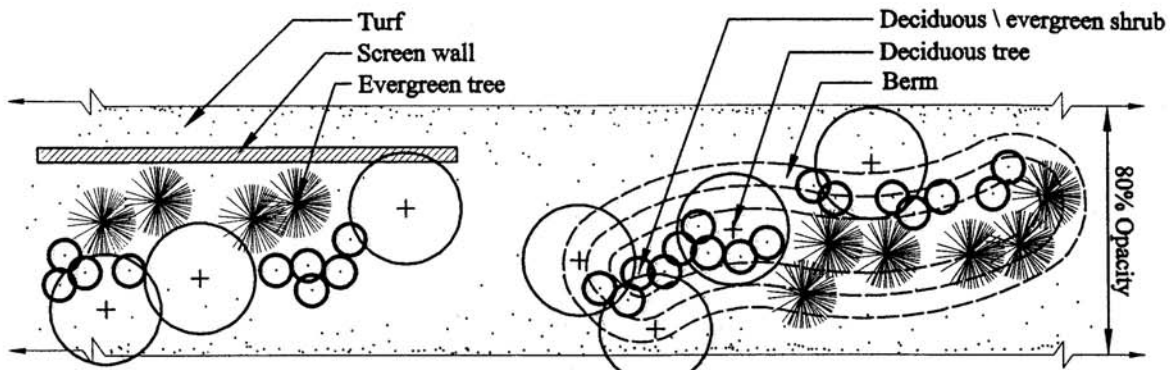
PLAN VIEW
