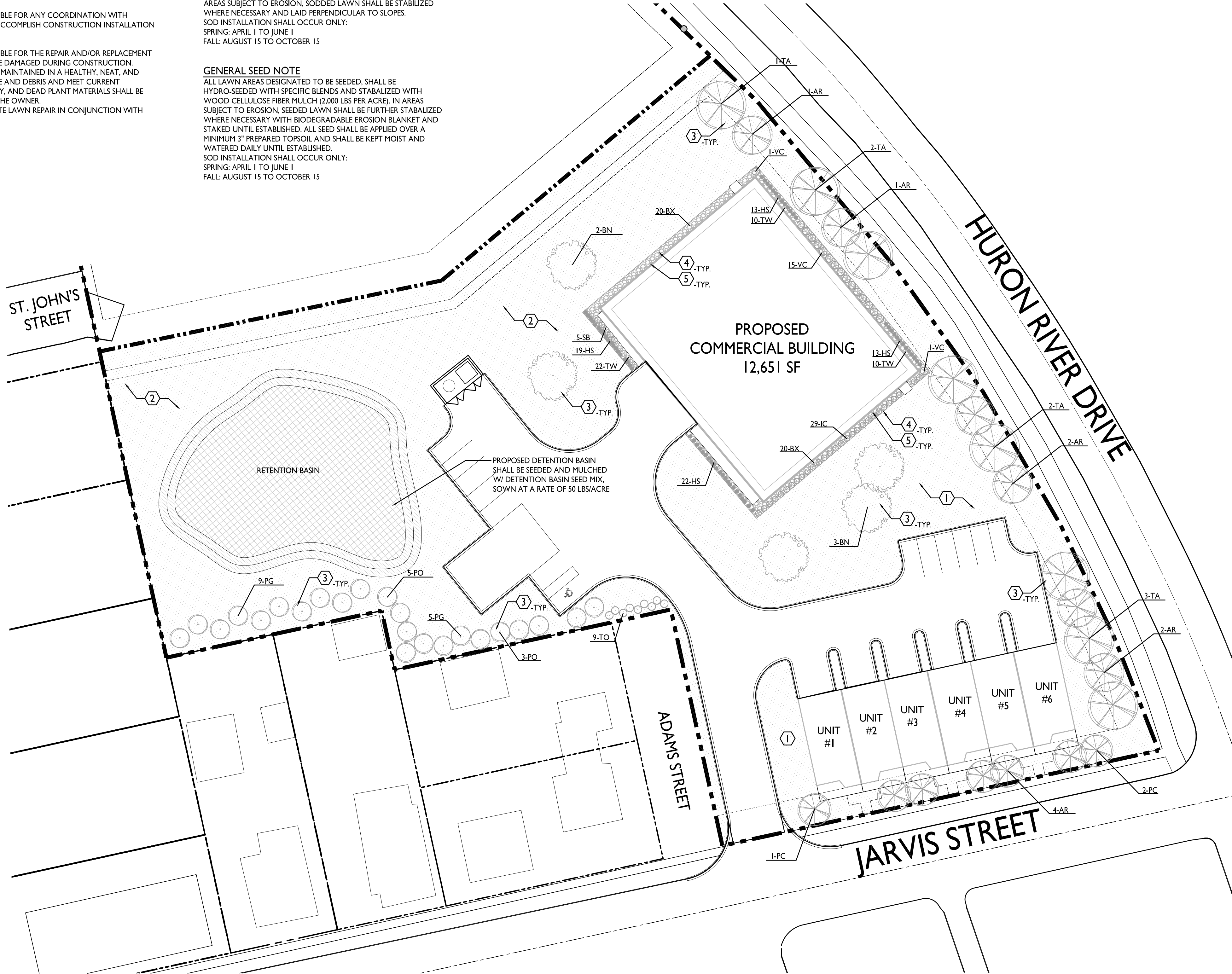
PRELIMINARY LANDSCAPE PLAN SCALE: 1" = 30'
