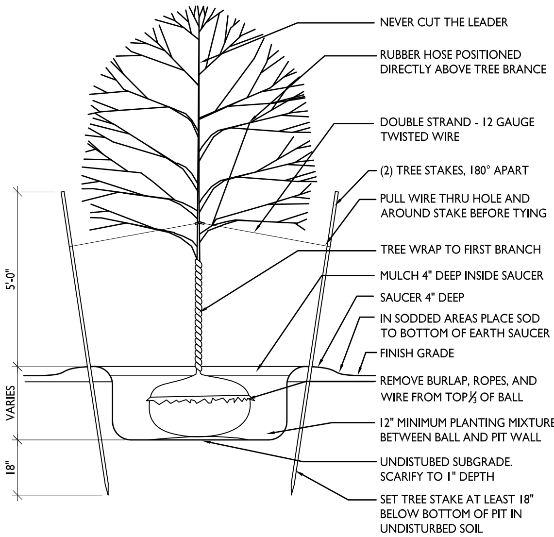
PLANTING DETAIL-DECIDUOUS NO SCALE
