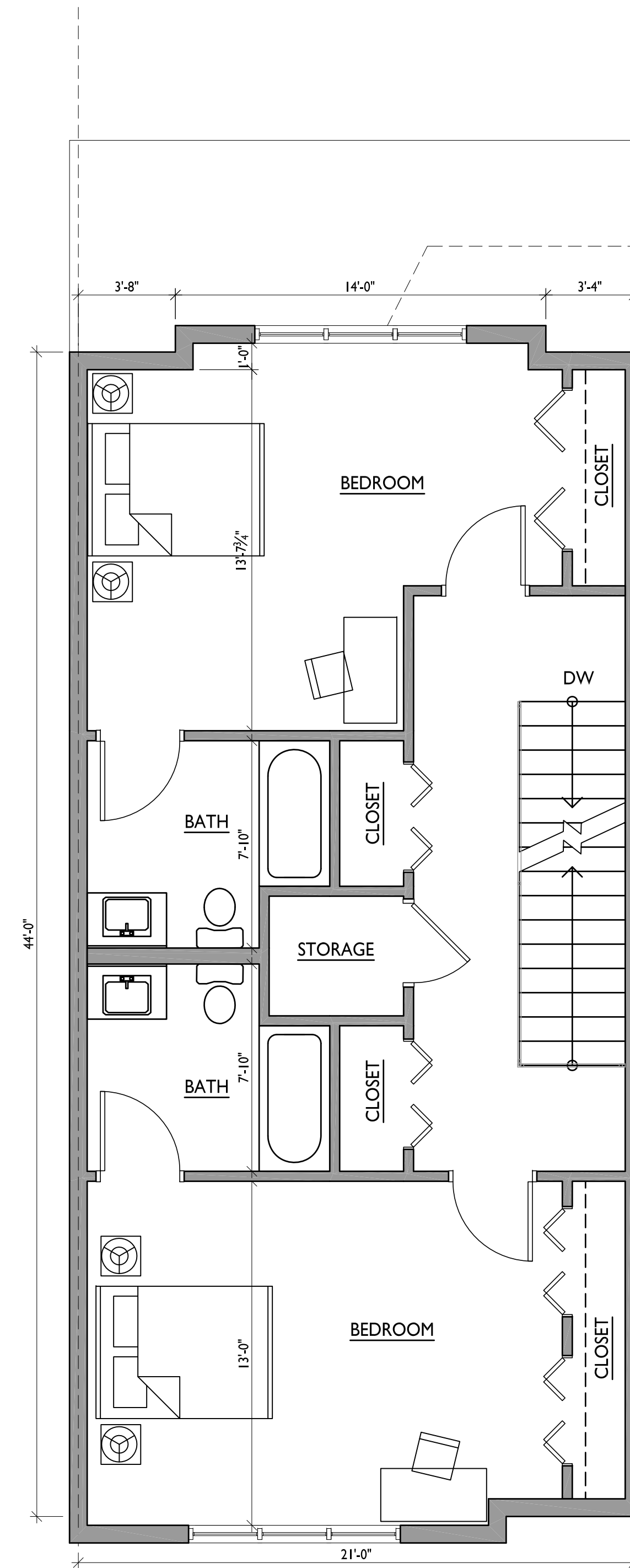
THIRD FLOOR PLAN (954 SQ. FT.) SCALE: 1/4"=1'-0"
