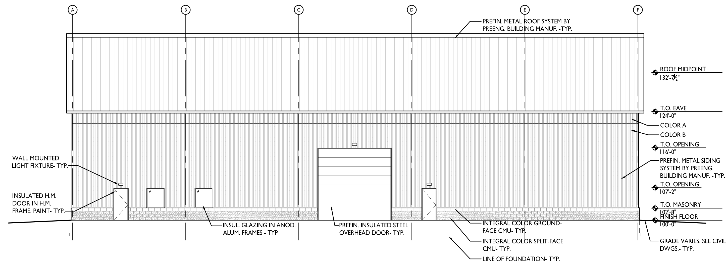
WEST ELEVATION
