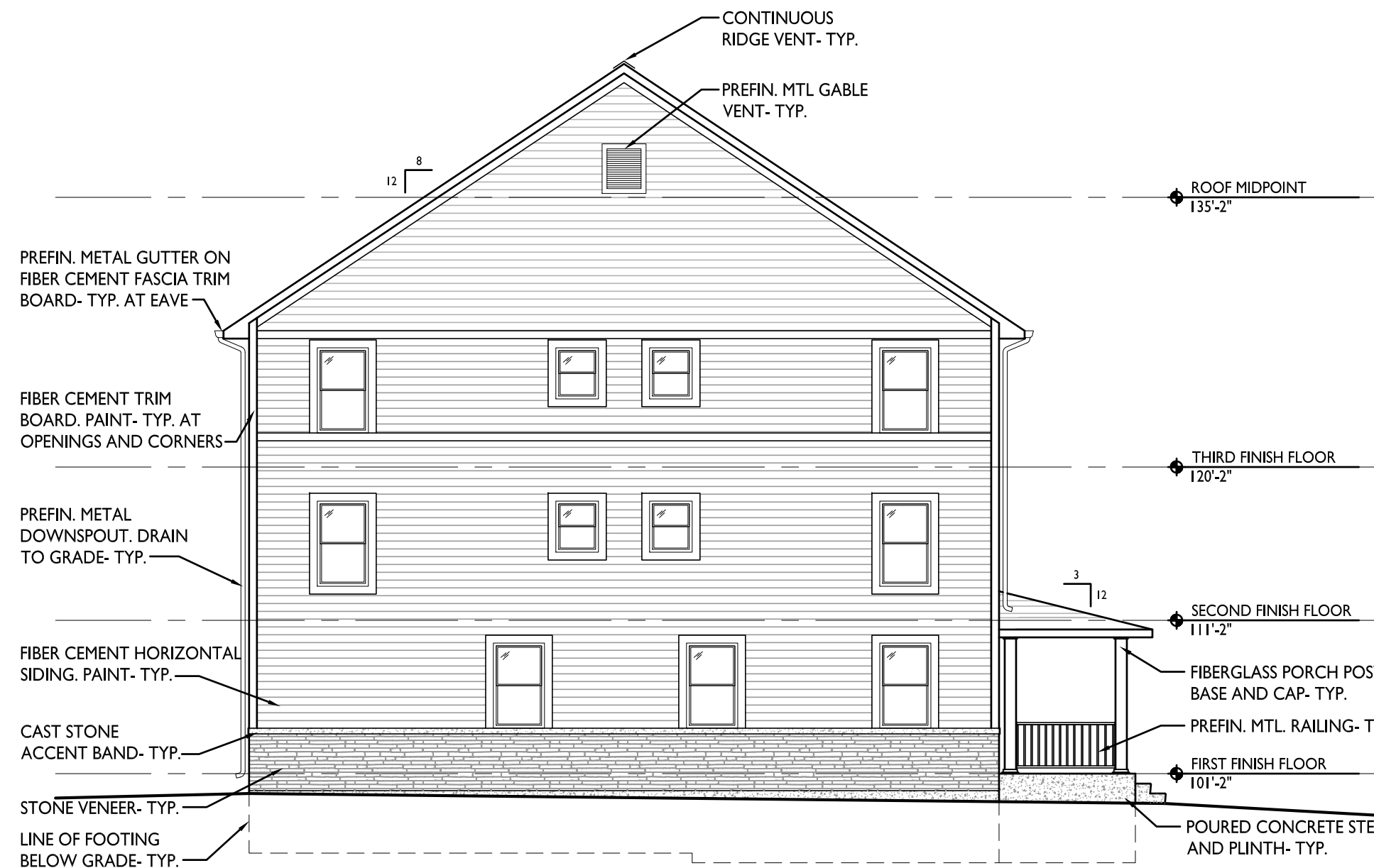
SIDE ELEVATION
