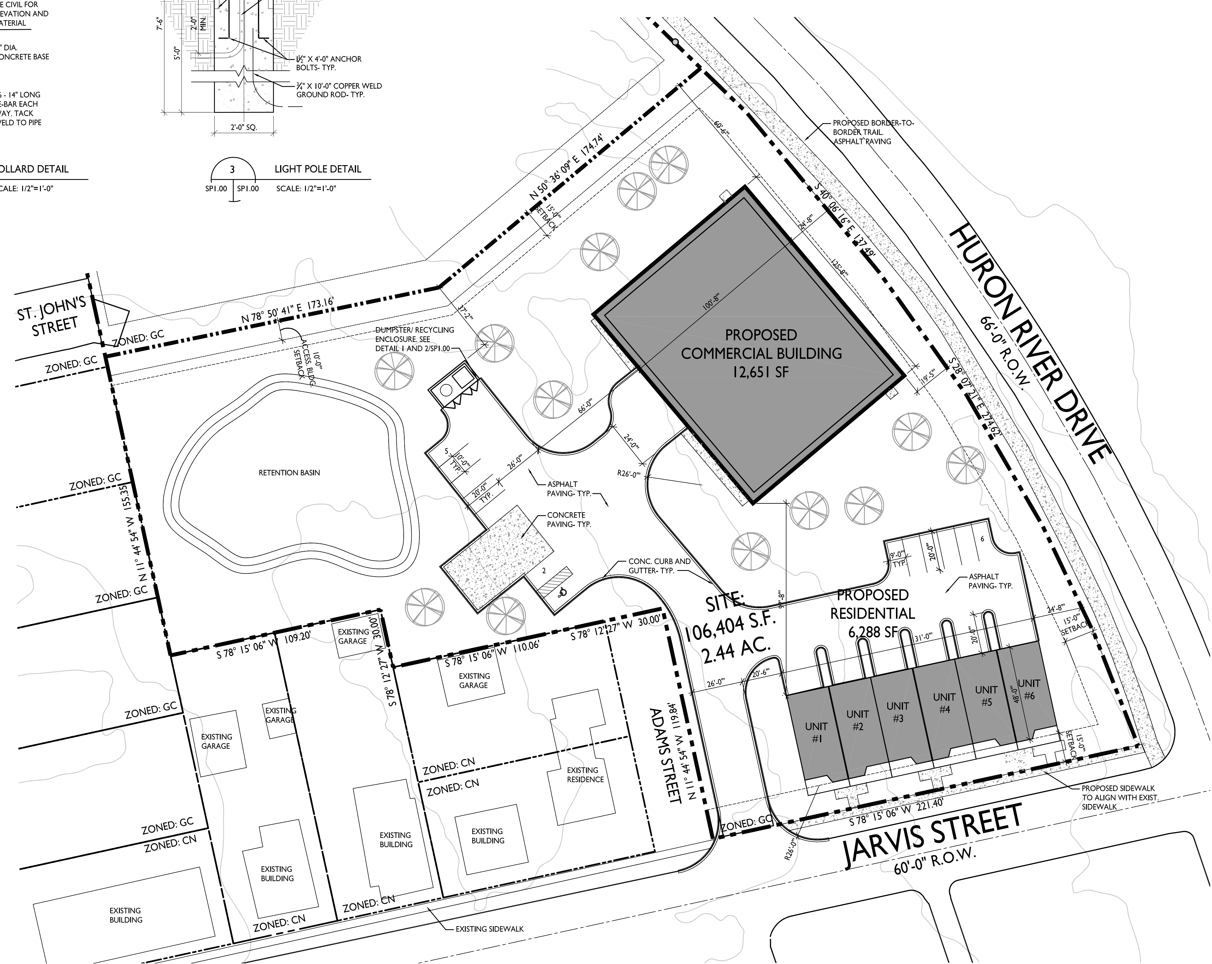
PRELIMINARY SITE PLAN SCALE: 1" = 30'
