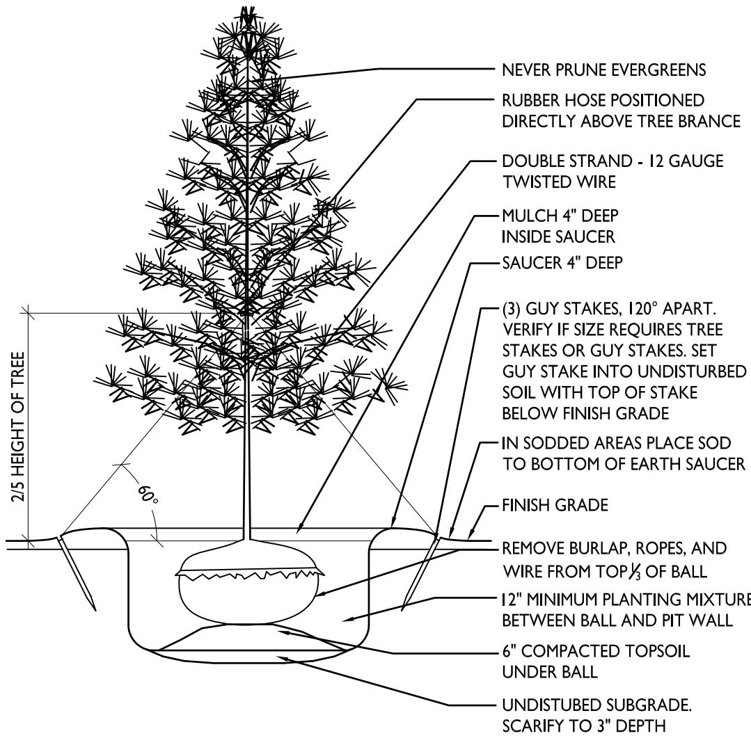
PLANTING DETAIL-EVERGREEN NO SCALE
