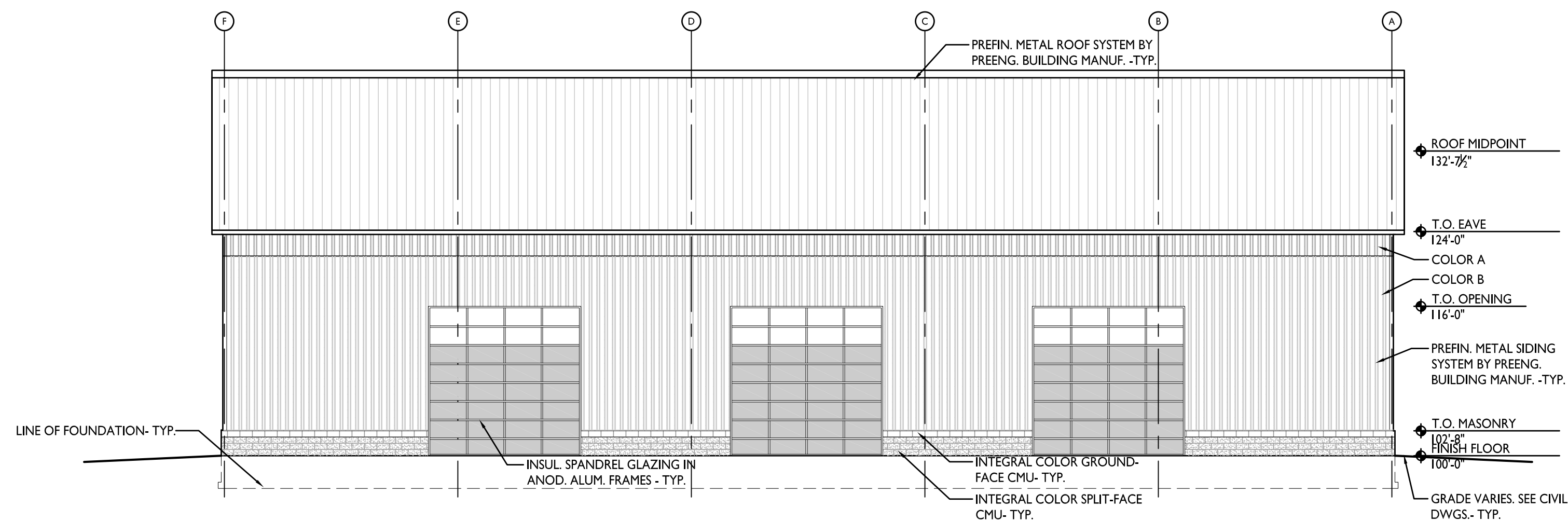
EAST ELEVATION
