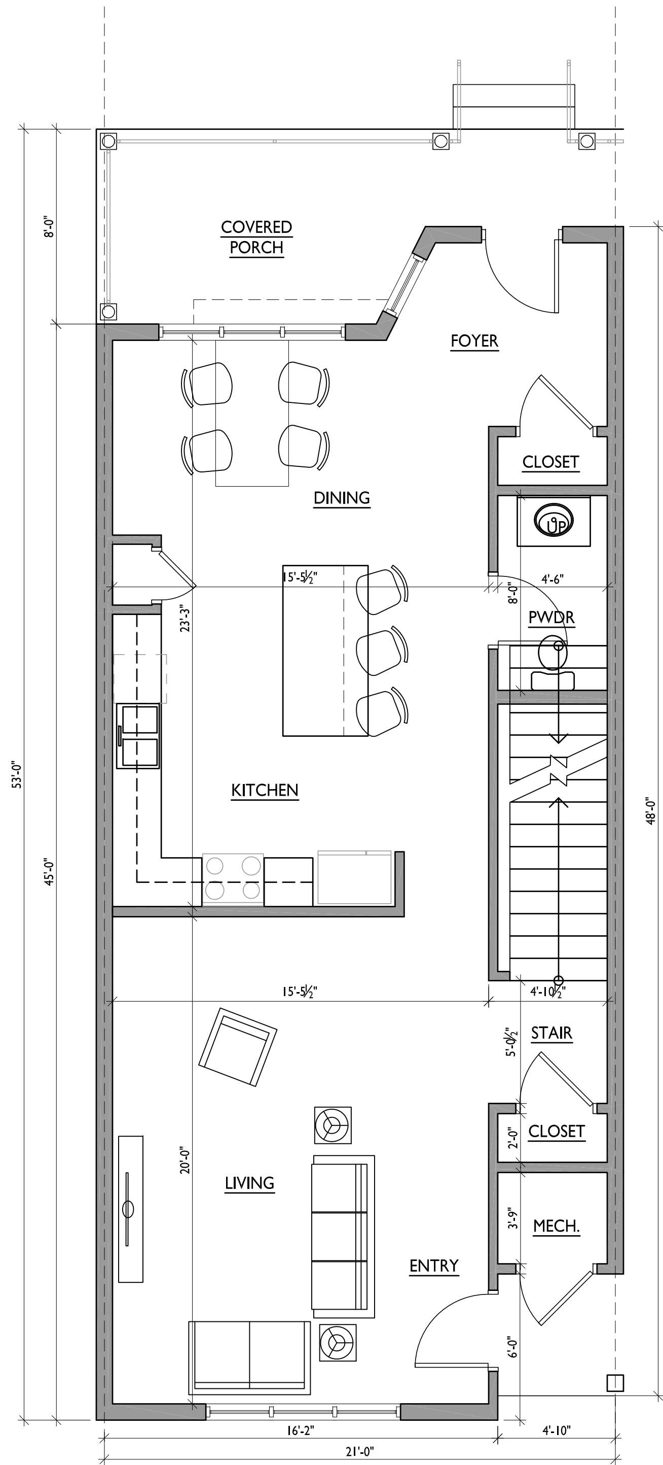
FIRST FLOOR PLAN (960 SQ. FT.) SCALE: 1/4"=1'-0"
