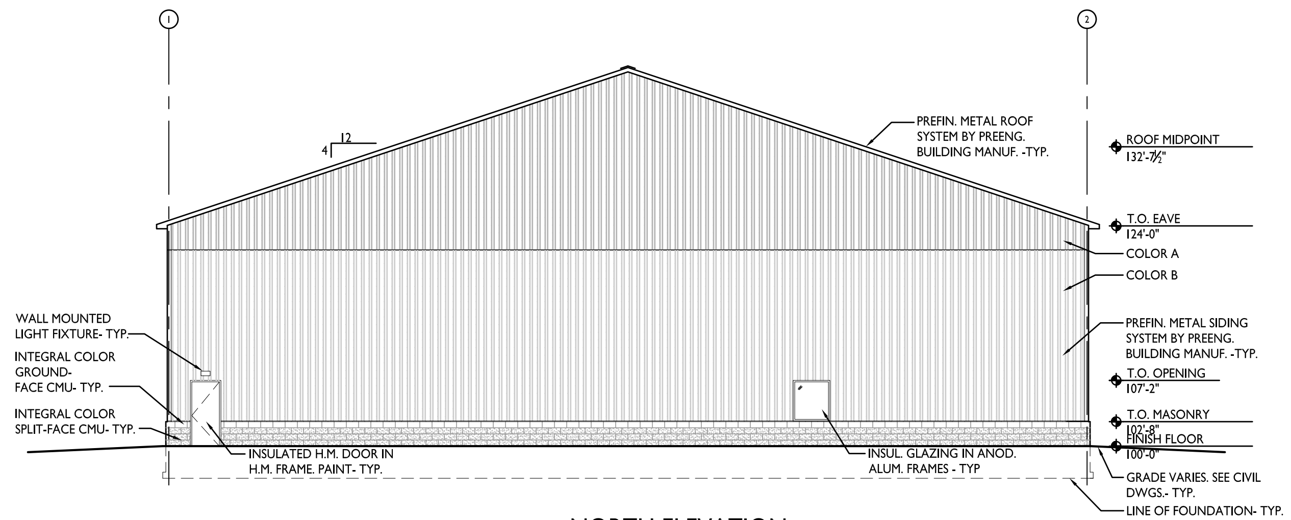
NORTH ELEVATION
